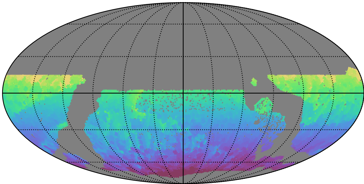
too_elab_r64_d3_giz_v3.4_10yrs WFD all bands: Min HA
