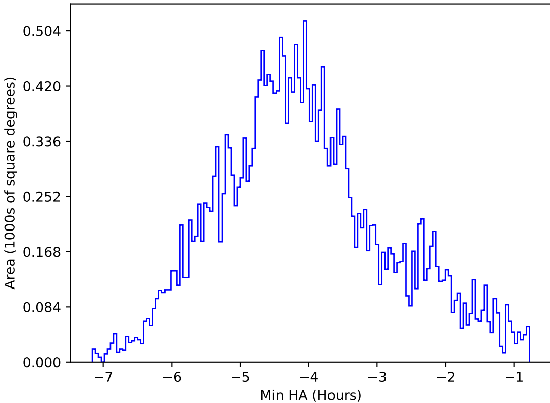
too_elab_r64_d3_giz_v3.4_10yrs All sky z band: Min HA
