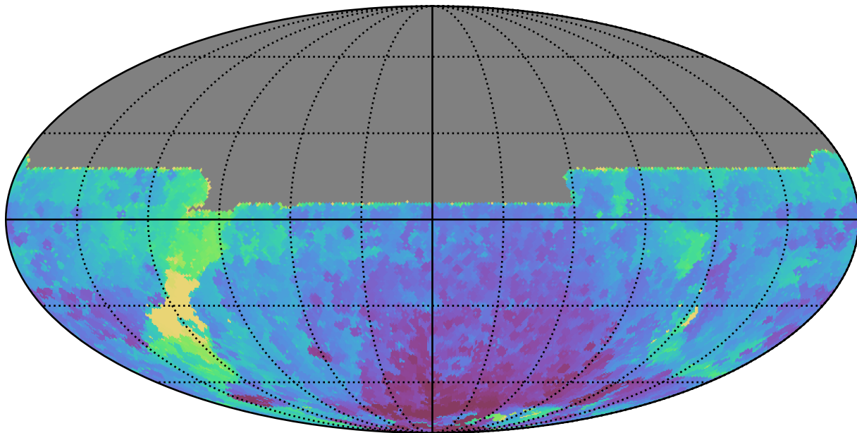
too_elab_r64_d3_giz_v3.4_10yrs All sky y band: Min HA
