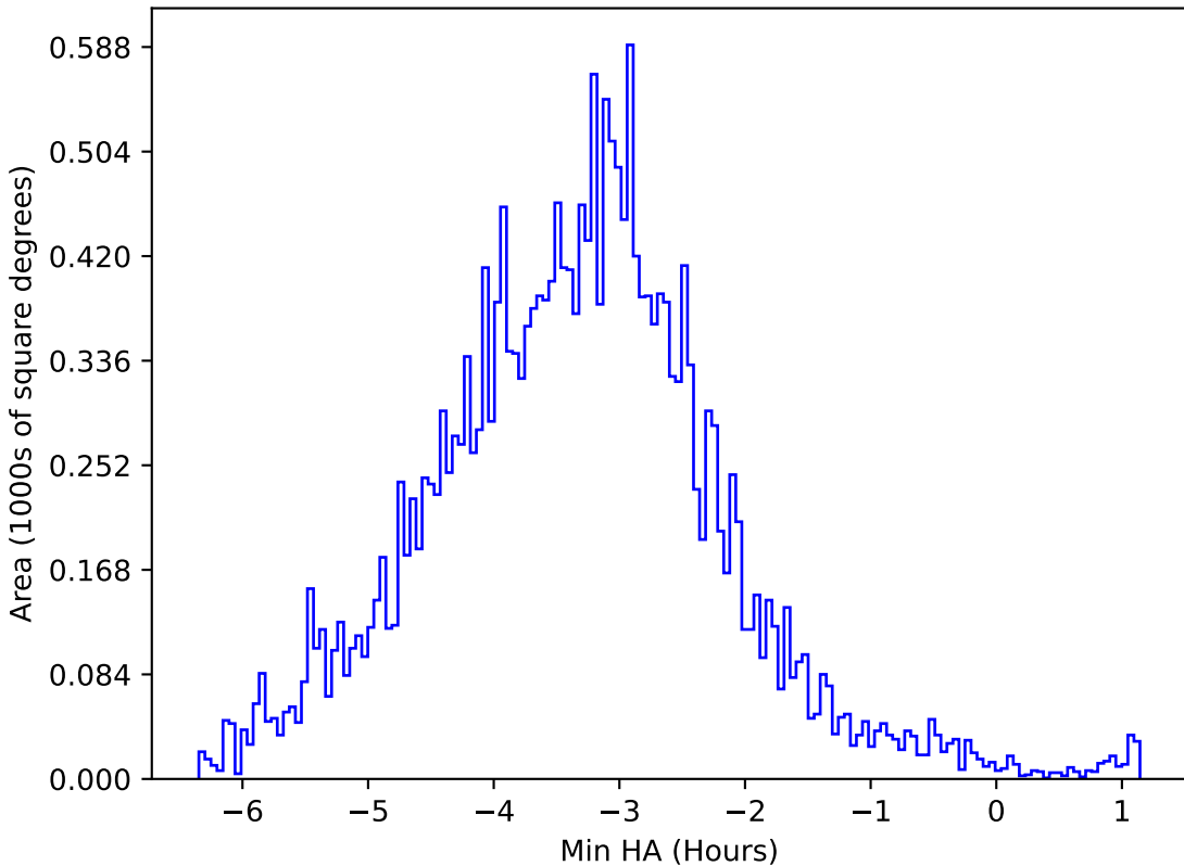
too_elab_r64_d3_giz_v3.4_10yrs All sky y band: Min HA
