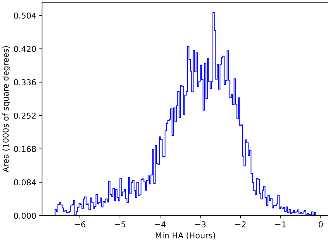
too_elab_r64_d3_giz_v3.4_10yrs All sky u band: Min HA
