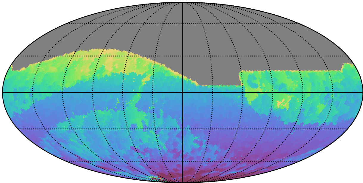
too_elab_r64_d3_giz_v3.4_10yrs All sky r band: Min HA
