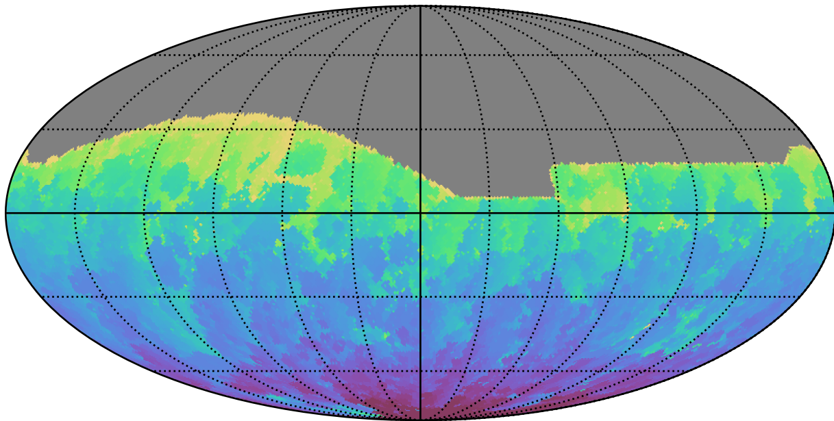
too_elab_r64_d3_giz_v3.4_10yrs All sky g band: Min HA
