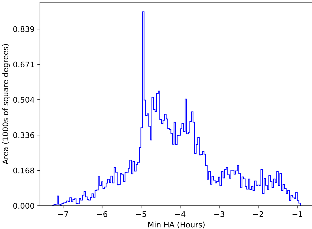
too_elab_r64_d3_giz_v3.4_10yrs All sky g band: Min HA
