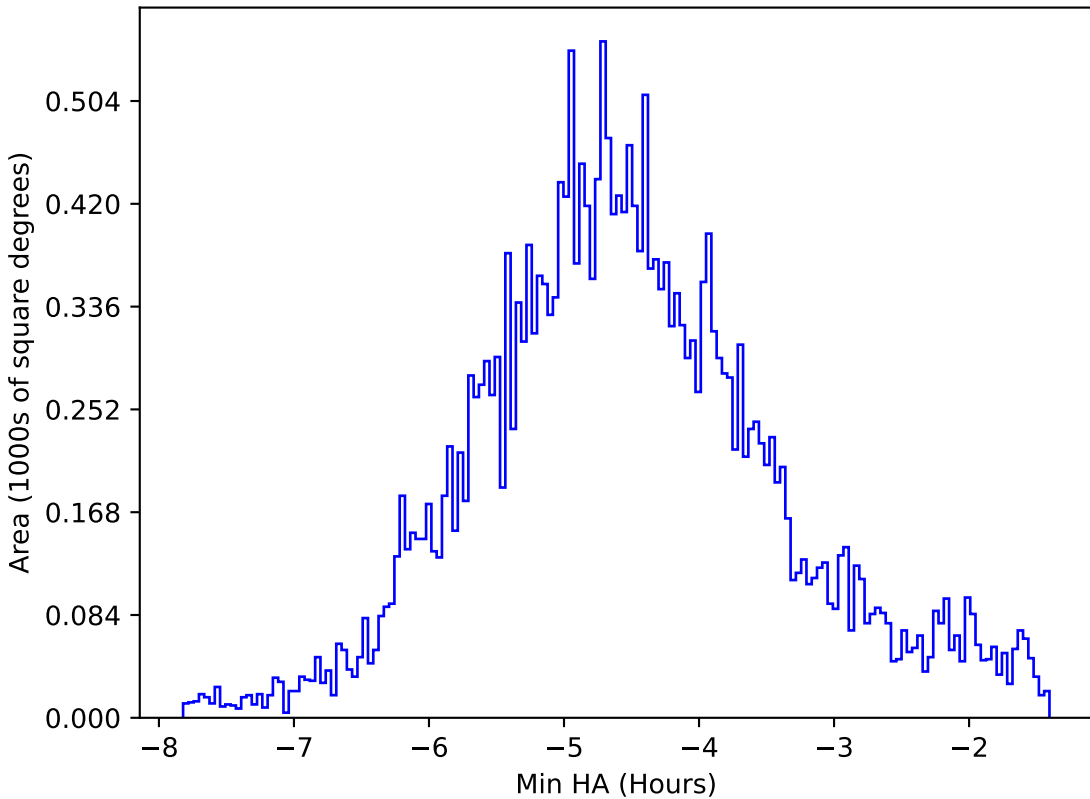
too_elab_r64_d3_giz_v3.4_10yrs All sky all bands: Min HA
