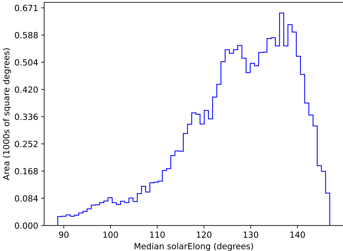
too_elab_r64_d3_giz_v3.4_10yrs WFD z band: Median solarElong
