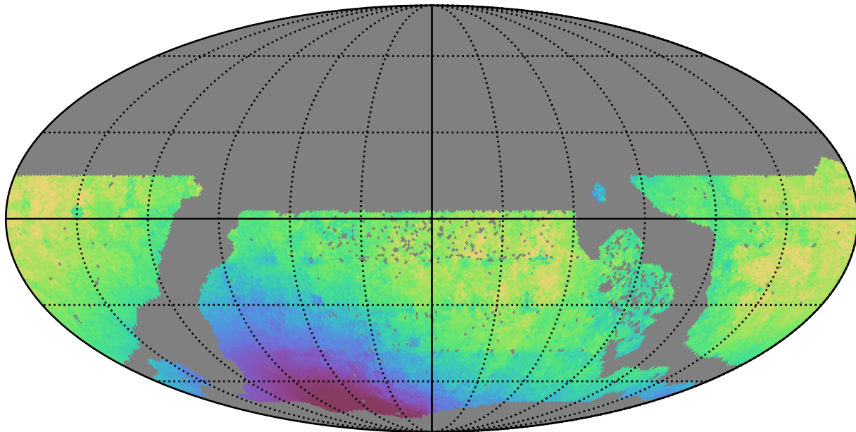
too_elab_r64_d3_giz_v3.4_10yrs WFD y band: Median solarElong
