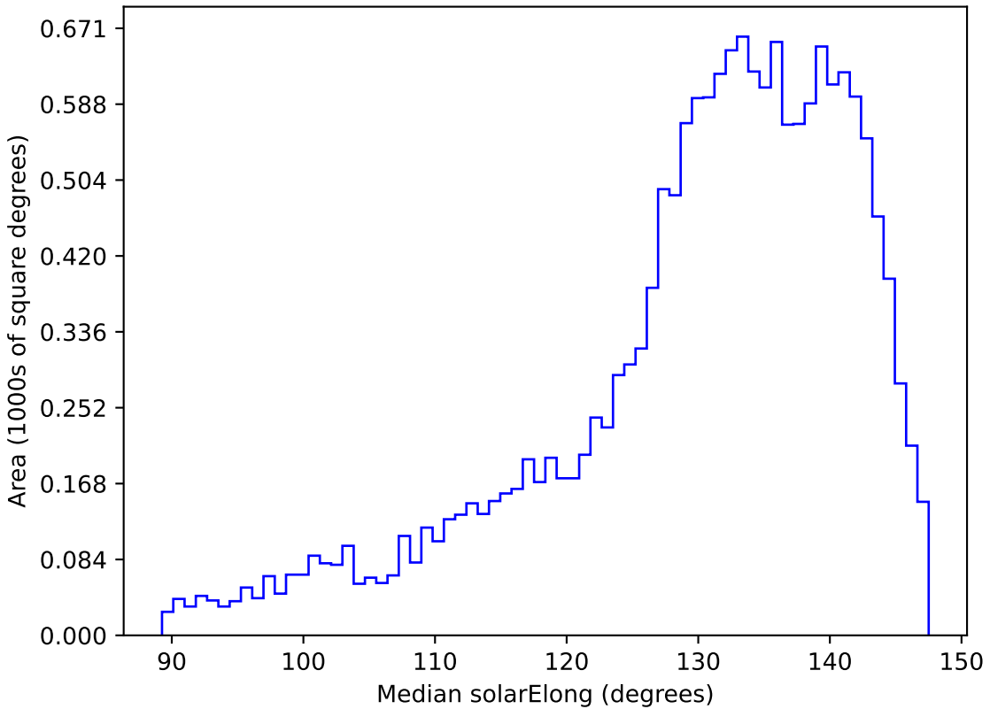
too_elab_r64_d3_giz_v3.4_10yrs WFD y band: Median solarElong
