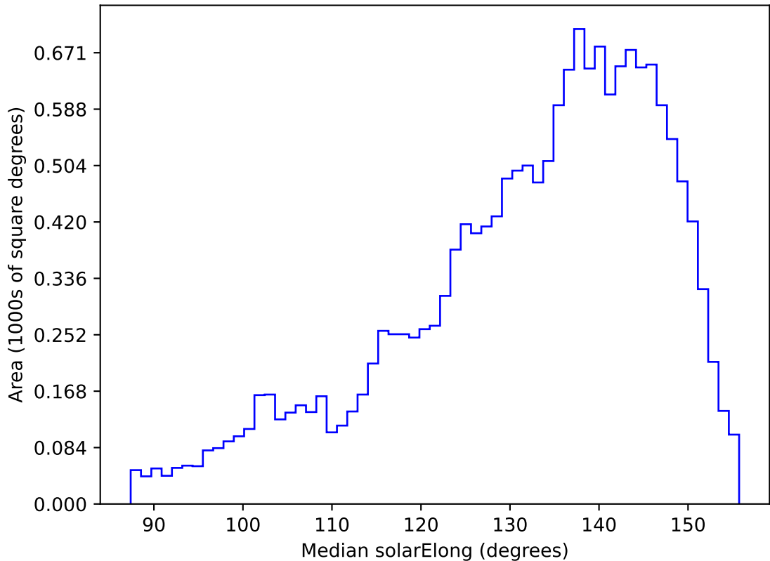
too_elab_r64_d3_giz_v3.4_10yrs WFD u band: Median solarElong
