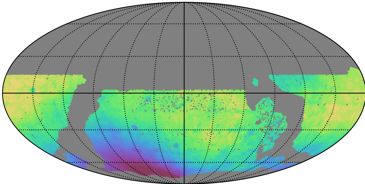
too_elab_r64_d3_giz_v3.4_10yrs WFD r band: Median solarElong
