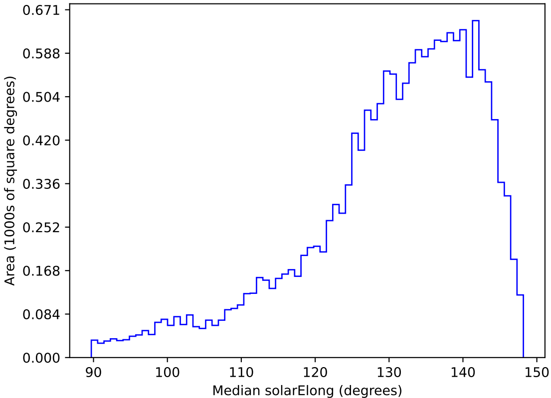
too_elab_r64_d3_giz_v3.4_10yrs WFD r band: Median solarElong
