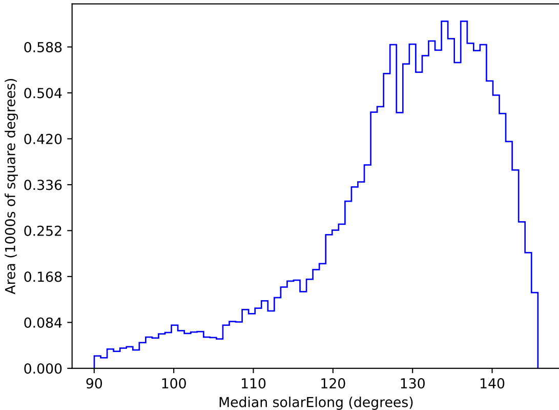
too_elab_r64_d3_giz_v3.4_10yrs WFD i band: Median solarElong
