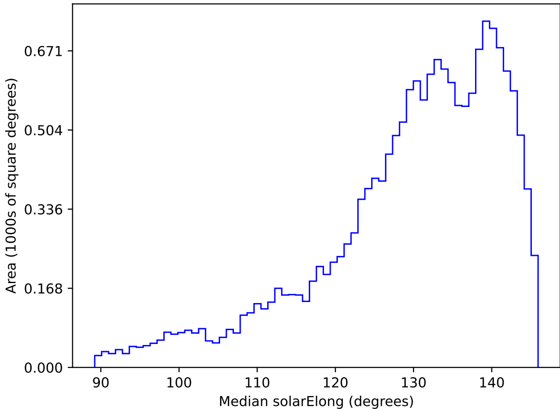
too_elab_r64_d3_giz_v3.4_10yrs WFD all bands: Median solarElong
