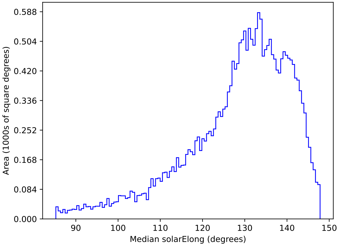
too_elab_r64_d3_giz_v3.4_10yrs All sky y band: Median solarElong
