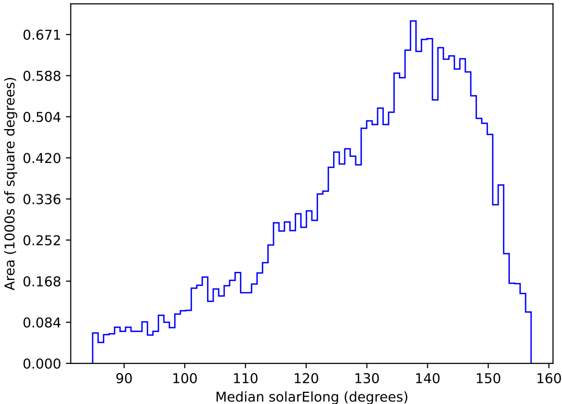
too_elab_r64_d3_giz_v3.4_10yrs All sky u band: Median solarElong
