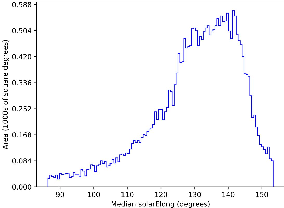
too_elab_r64_d3_giz_v3.4_10yrs All sky r band: Median solarElong
