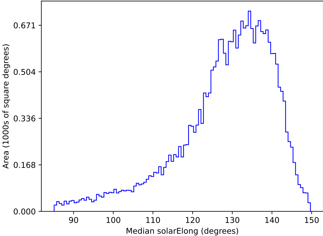
too_elab_r64_d3_giz_v3.4_10yrs All sky i band: Median solarElong
