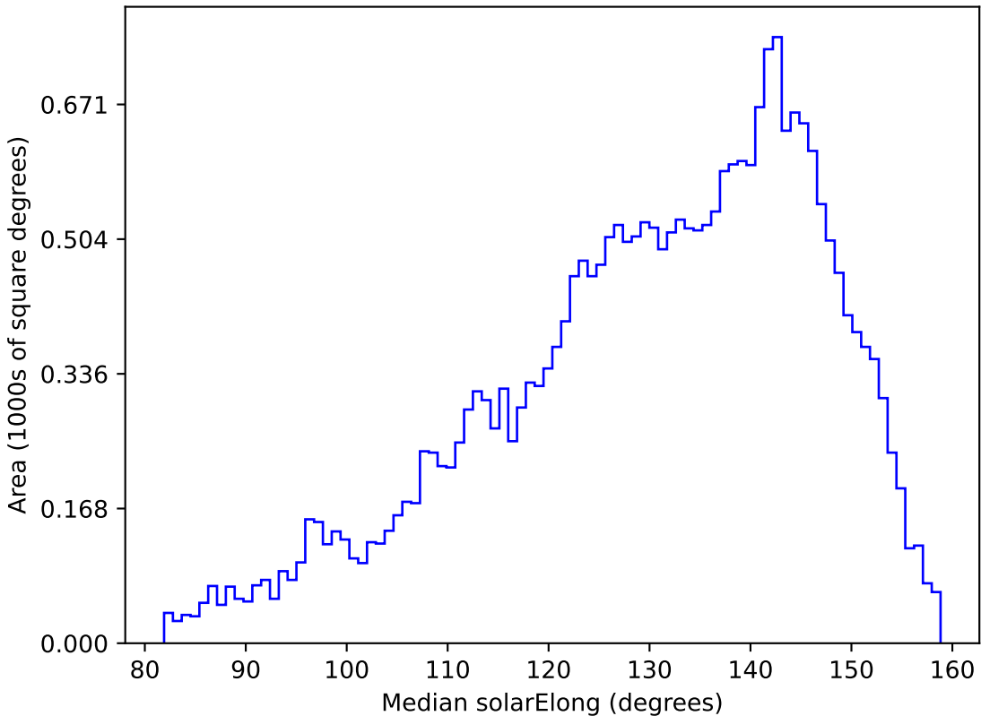
too_elab_r64_d3_giz_v3.4_10yrs All sky g band: Median solarElong
