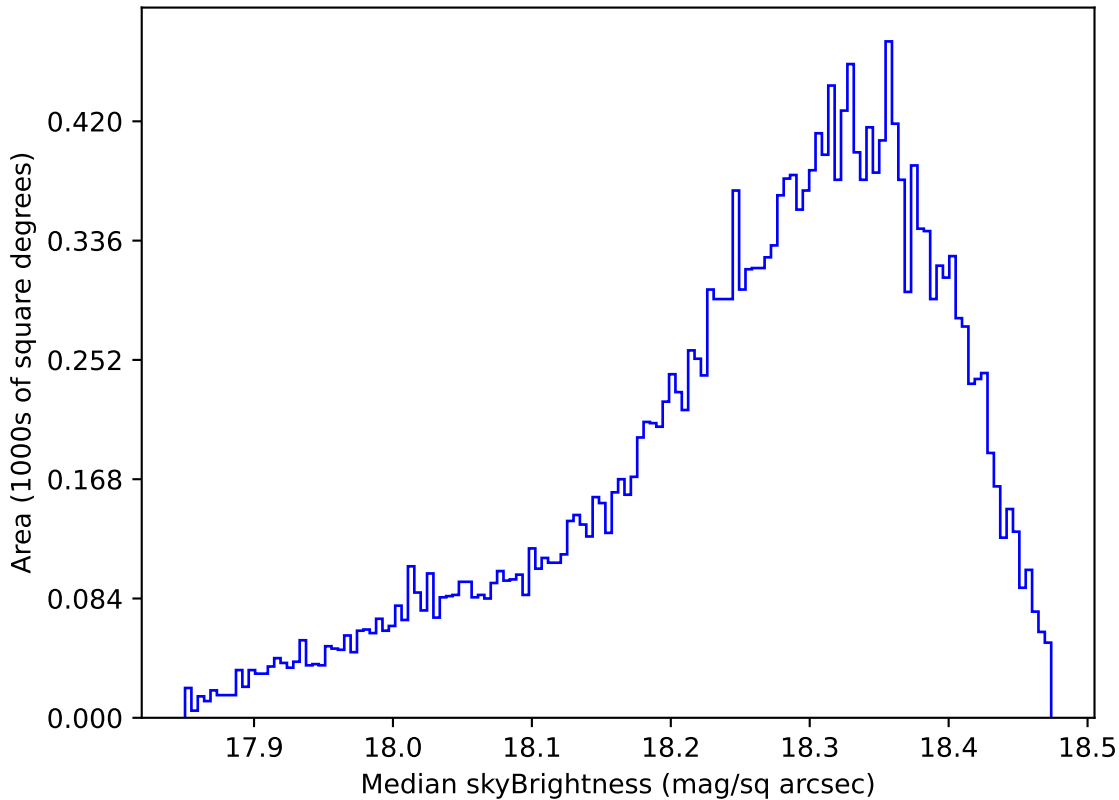
too_elab_r64_d3_giz_v3.4_10yrs Yr 1 y band: Median skyBrightness
