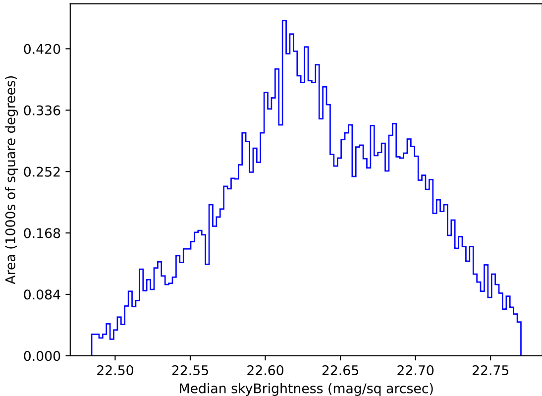
too_elab_r64_d3_giz_v3.4_10yrs Yr 1 u band: Median skyBrightness
