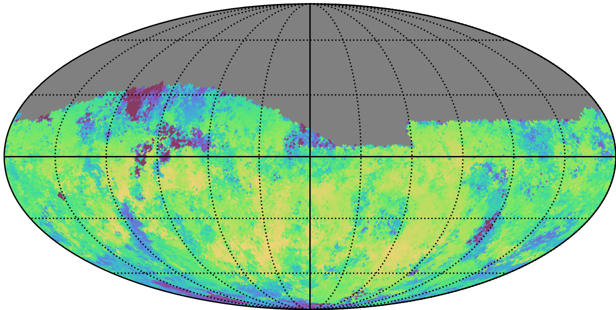
too_elab_r64_d3_giz_v3.4_10yrs Yr 1 i band: Median skyBrightness
