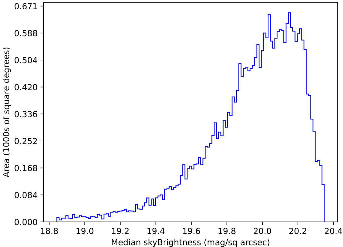
too_elab_r64_d3_giz_v3.4_10yrs Yr 1 i band: Median skyBrightness
