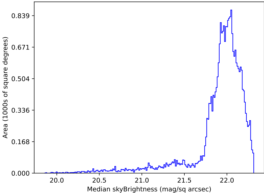
too_elab_r64_d3_giz_v3.4_10yrs Yr 1 g band: Median skyBrightness
