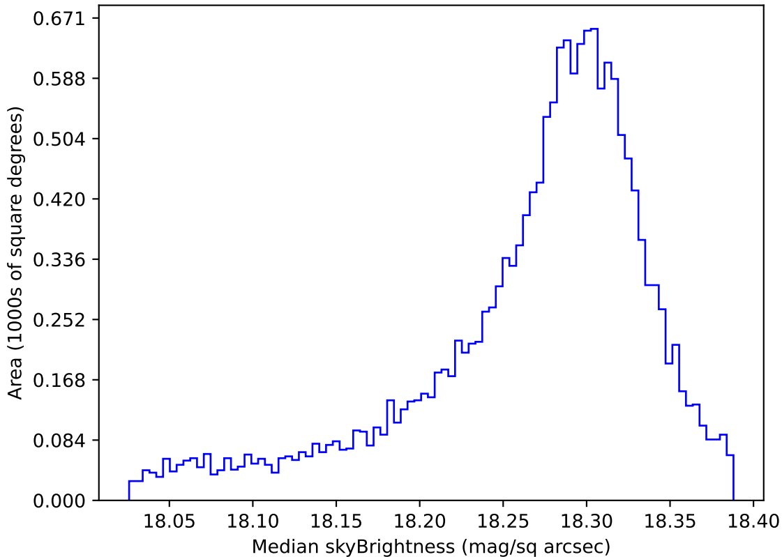
too_elab_r64_d3_giz_v3.4_10yrs WFD y band: Median skyBrightness
