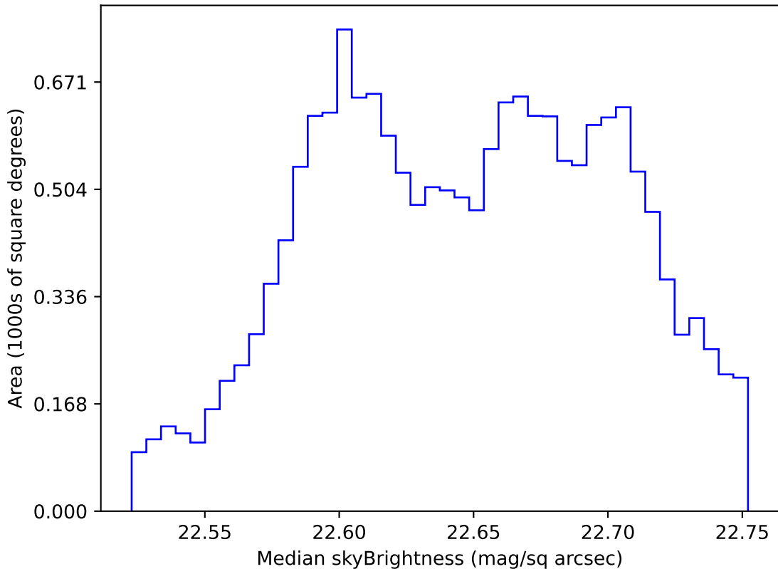
too_elab_r64_d3_giz_v3.4_10yrs WFD u band: Median skyBrightness
