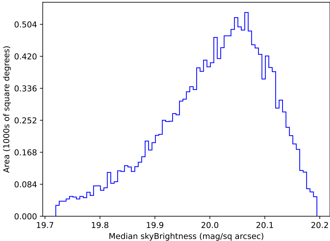
too_elab_r64_d3_giz_v3.4_10yrs WFD i band: Median skyBrightness
