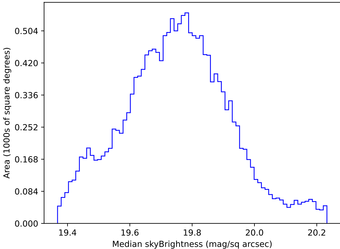
too_elab_r64_d3_giz_v3.4_10yrs WFD all bands: Median skyBrightness
