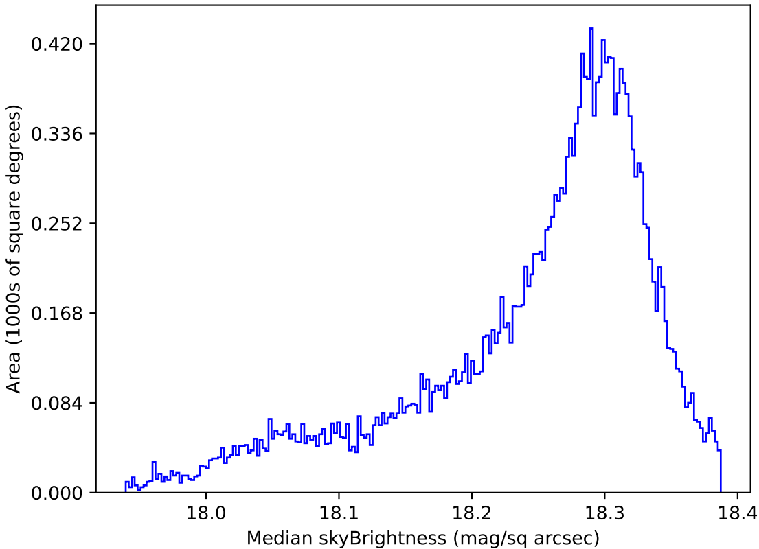
too_elab_r64_d3_giz_v3.4_10yrs All sky y band: Median skyBrightness
