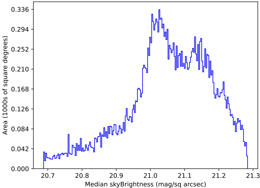
too_elab_r64_d3_giz_v3.4_10yrs All sky r band: Median skyBrightness
