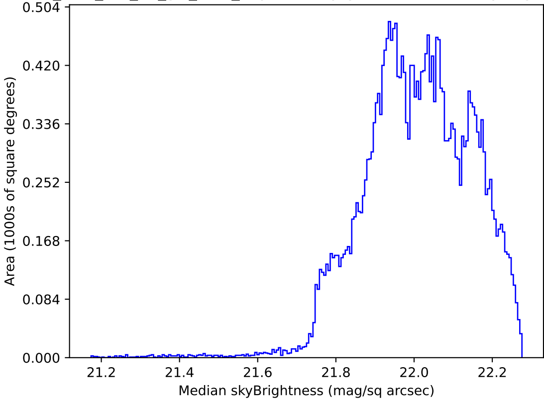
too_elab_r64_d3_giz_v3.4_10yrs All sky g band: Median skyBrightness
