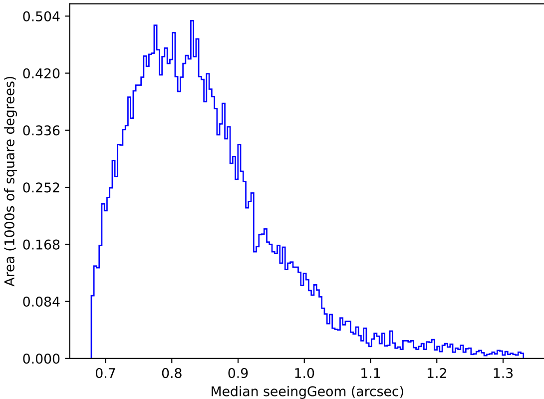
too_elab_r64_d3_giz_v3.4_10yrs Yr 1 z band: Median seeingGeom
