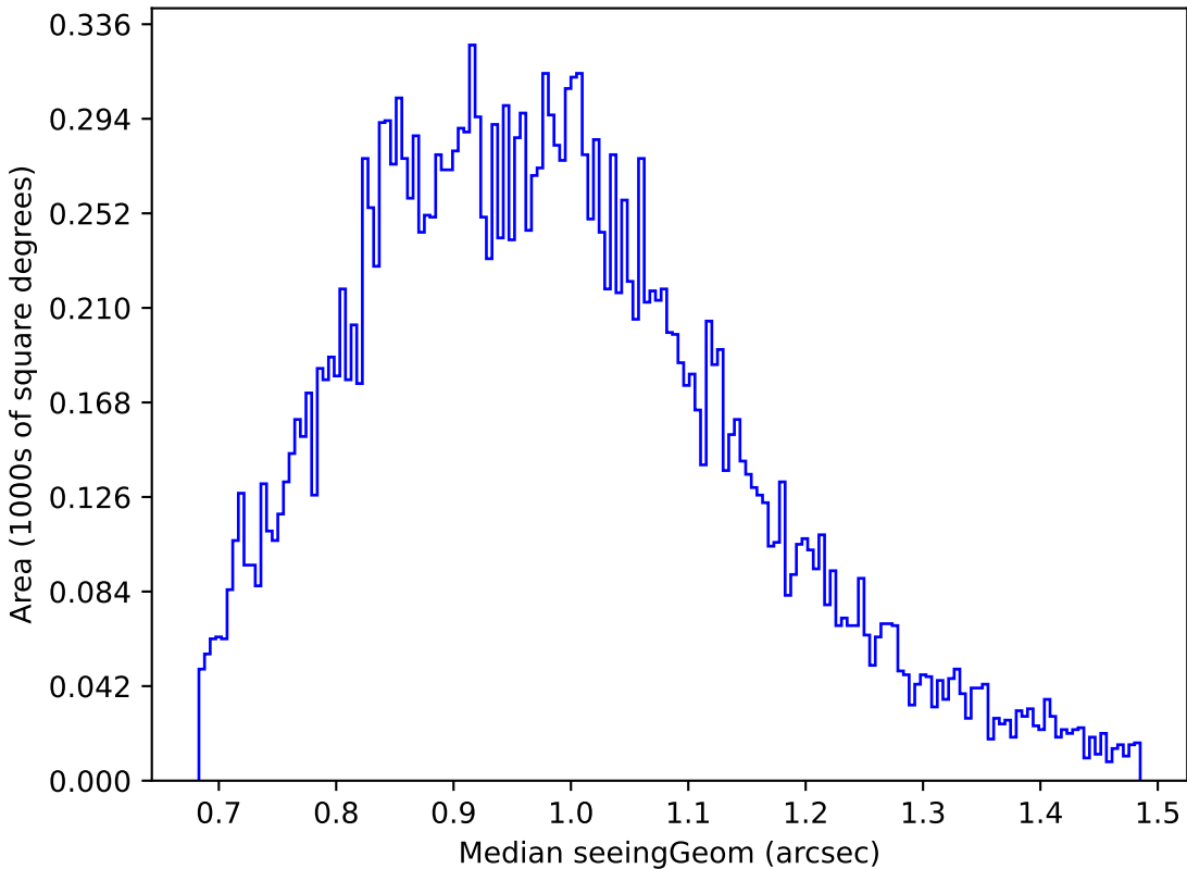
too_elab_r64_d3_giz_v3.4_10yrs Yr 1 u band: Median seeingGeom
