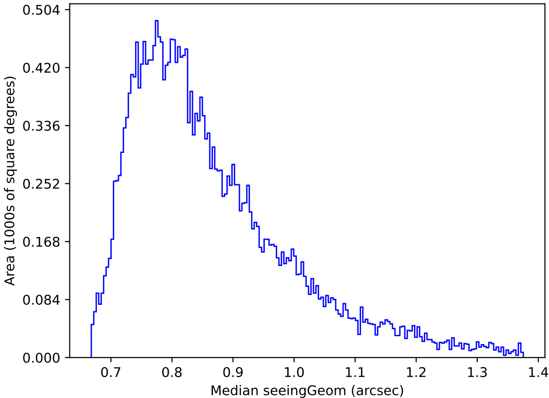
too_elab_r64_d3_giz_v3.4_10yrs Yr 1 r band: Median seeingGeom
