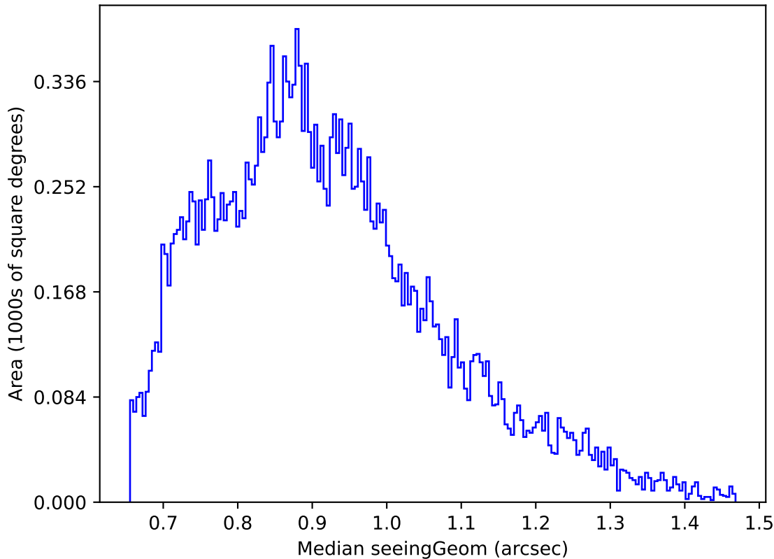
too_elab_r64_d3_giz_v3.4_10yrs Yr 1 g band: Median seeingGeom
