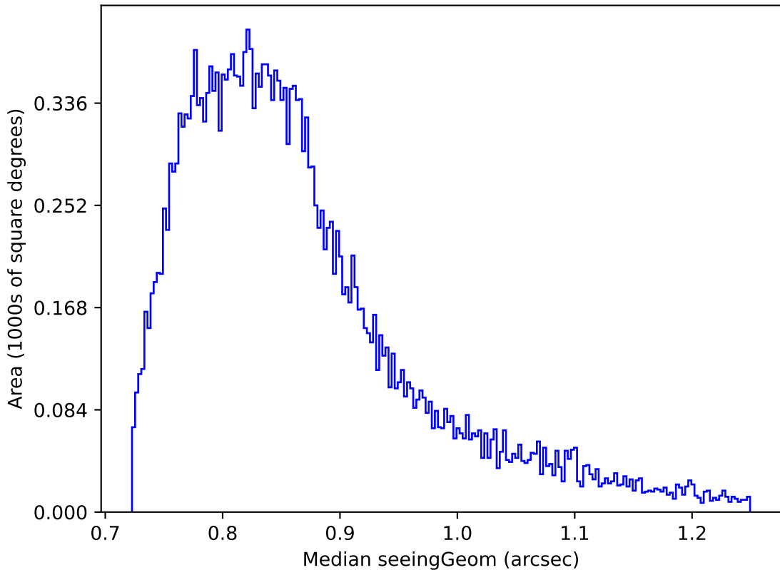
too_elab_r64_d3_giz_v3.4_10yrs Yr 1 all bands: Median seeingGeom
