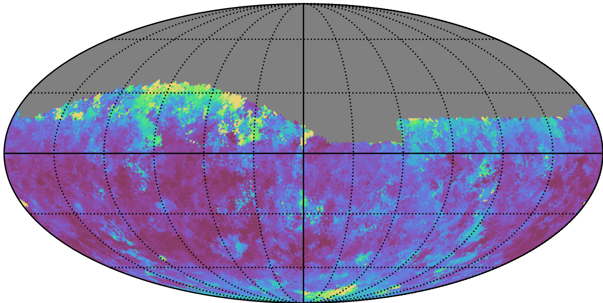
too_elab_r64_d3_giz_v3.4_10yrs Yr 1 z band: Median seeingEff
