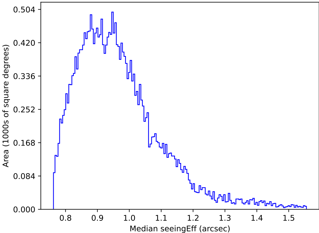
too_elab_r64_d3_giz_v3.4_10yrs Yr 1 z band: Median seeingEff
