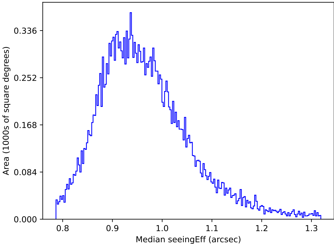
too_elab_r64_d3_giz_v3.4_10yrs Yr 1 y band: Median seeingEff
