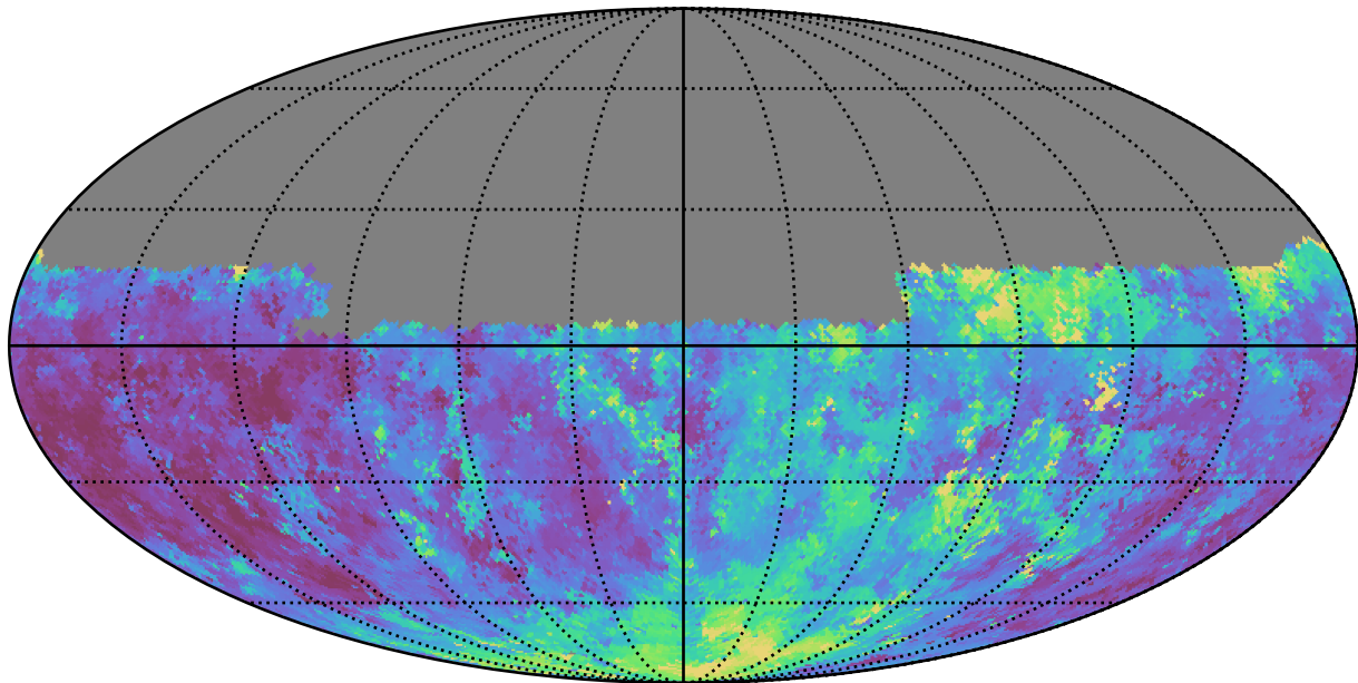
too_elab_r64_d3_giz_v3.4_10yrs Yr 1 u band: Median seeingEff
