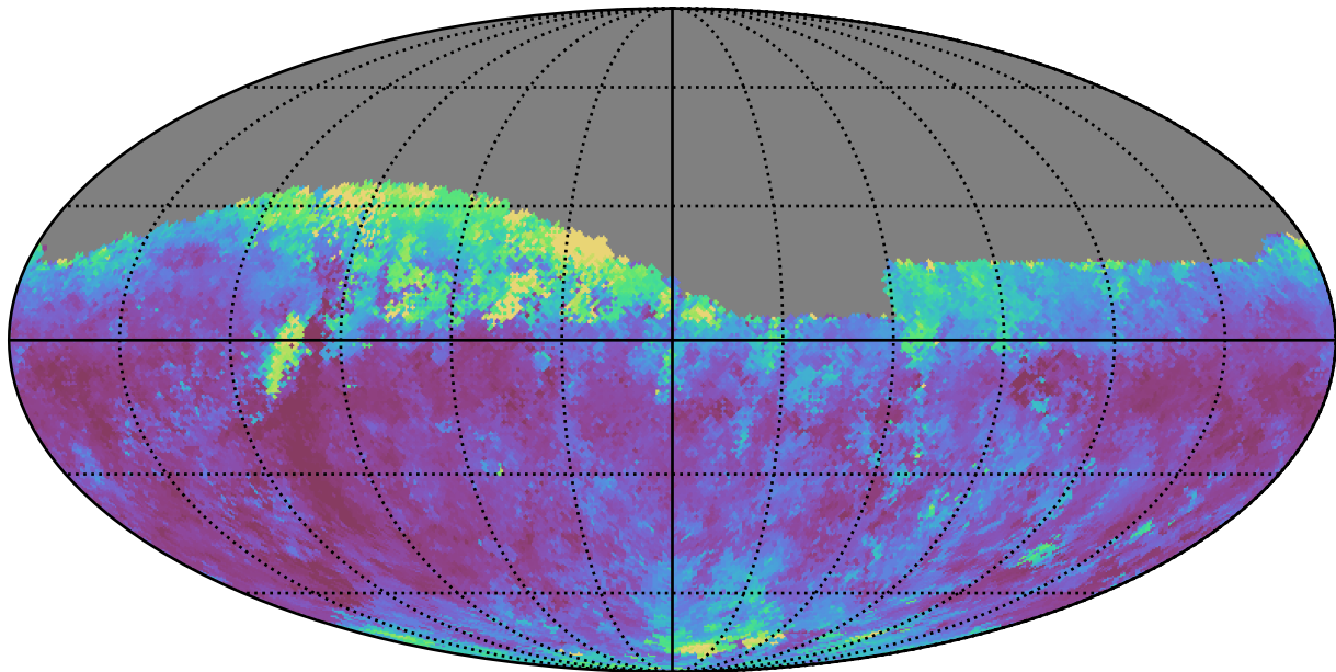
too_elab_r64_d3_giz_v3.4_10yrs Yr 1 r band: Median seeingEff
