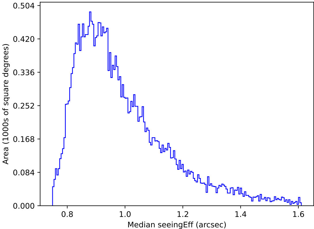
too_elab_r64_d3_giz_v3.4_10yrs Yr 1 r band: Median seeingEff
