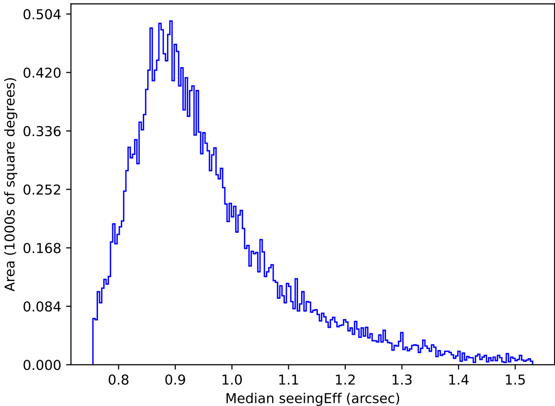
too_elab_r64_d3_giz_v3.4_10yrs Yr 1 i band: Median seeingEff
