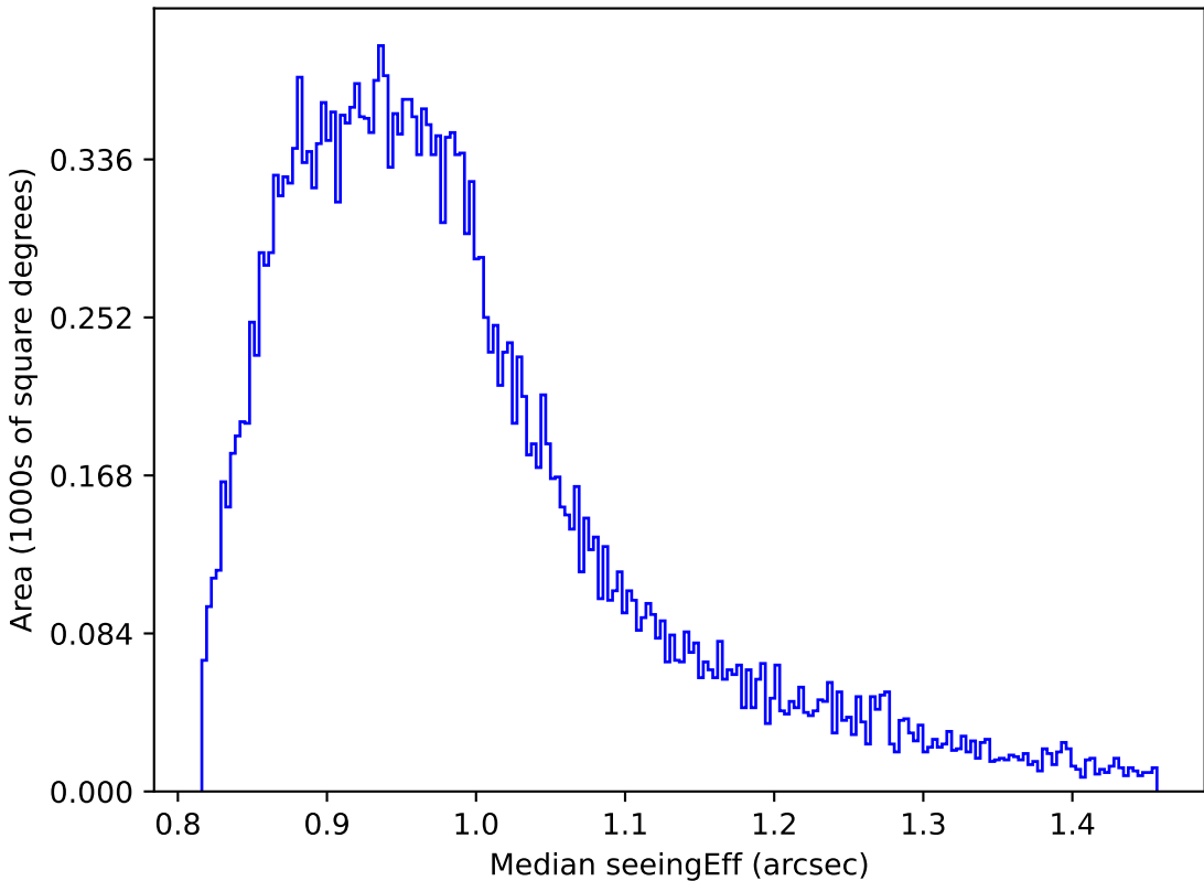
too_elab_r64_d3_giz_v3.4_10yrs Yr 1 all bands: Median seeingEff
