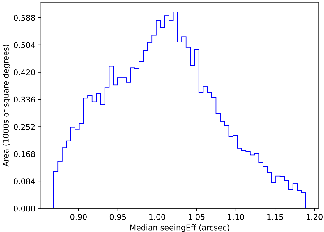
too_elab_r64_d3_giz_v3.4_10yrs WFD z band: Median seeingEff
