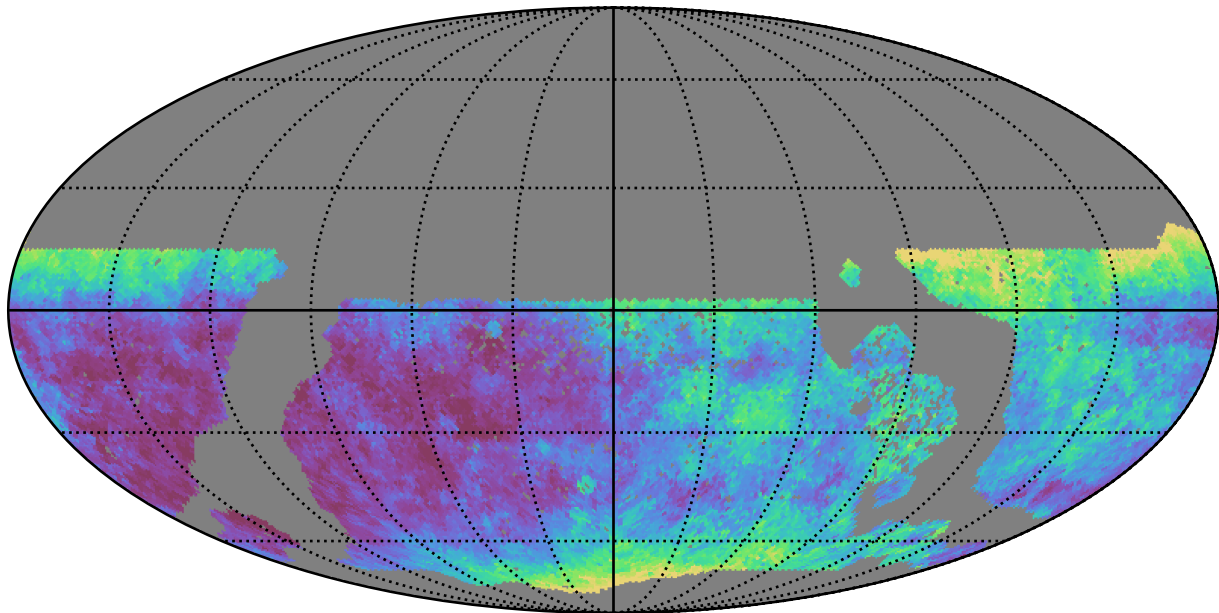
too_elab_r64_d3_giz_v3.4_10yrs WFD y band: Median seeingEff
