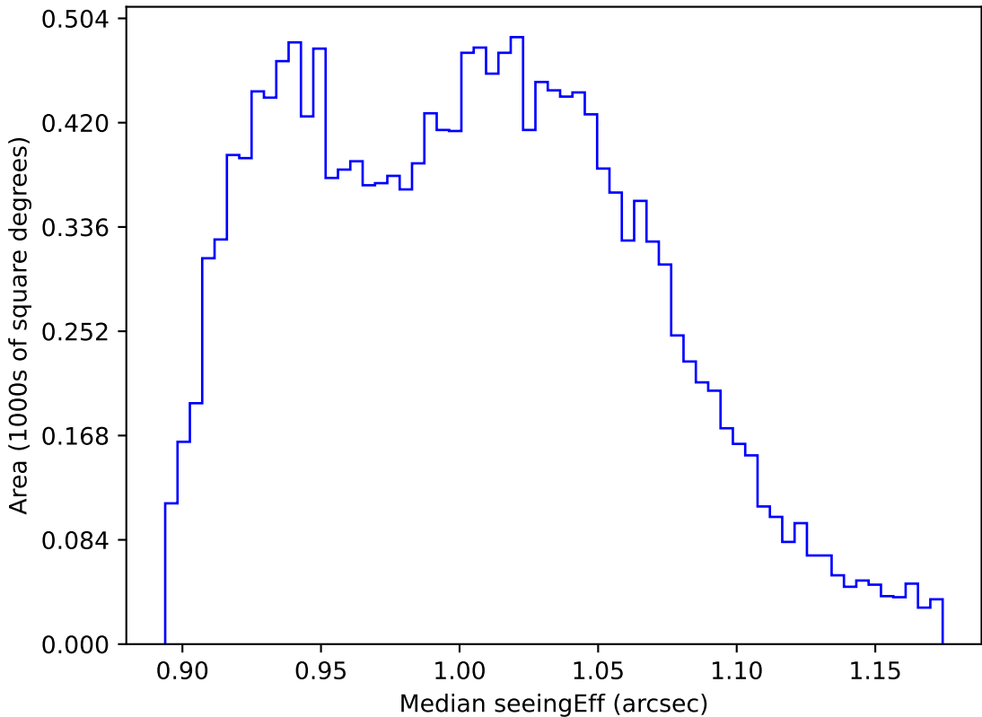
too_elab_r64_d3_giz_v3.4_10yrs WFD y band: Median seeingEff
